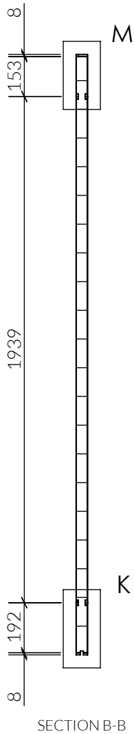
SECTION B-B
