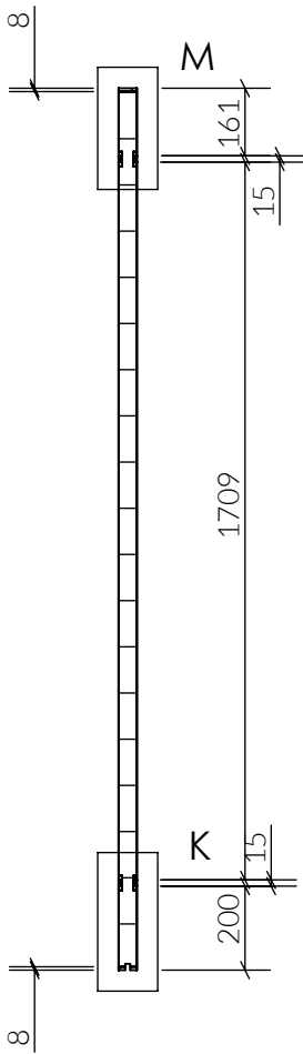
SECTION B-B
