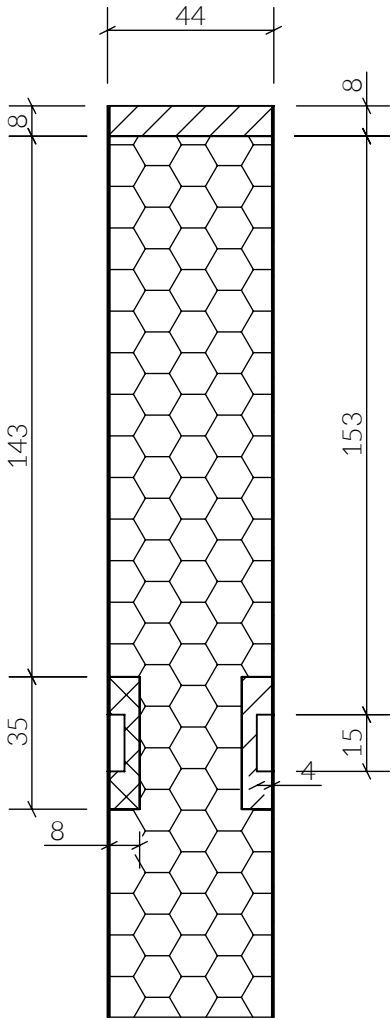
DETAIL M SCALE 1:2
