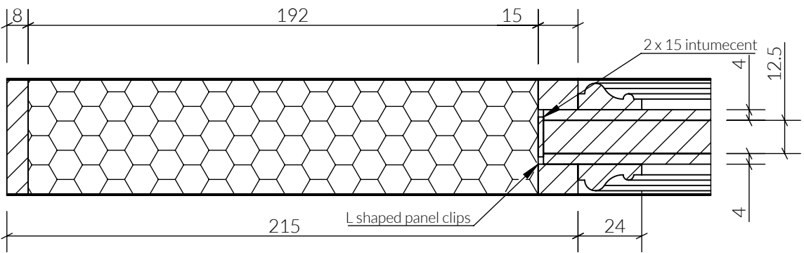
DETAIL N SCALE 1:2
