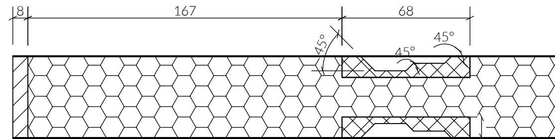
DETAIL N SCALE 1 : 2
