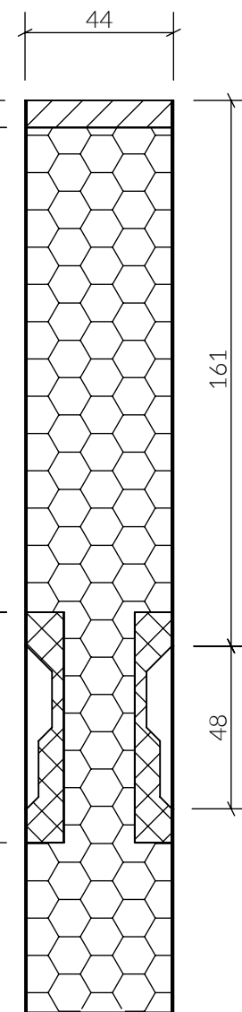
DETAIL M SCALE 1 : 2
