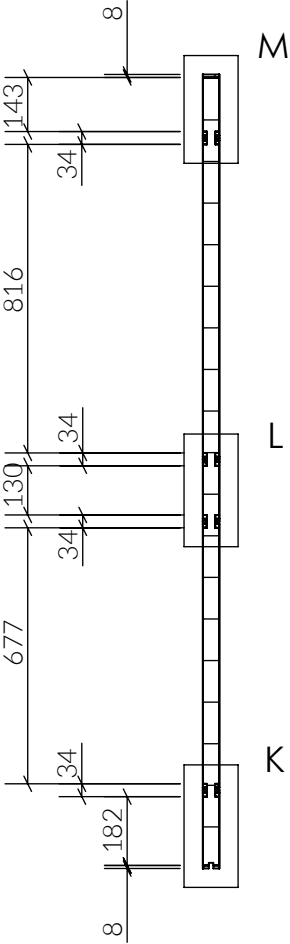
SECTION B-B
